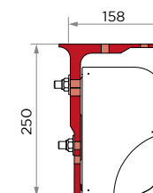
Quartz & Quartz Lux - Pose plafond -
